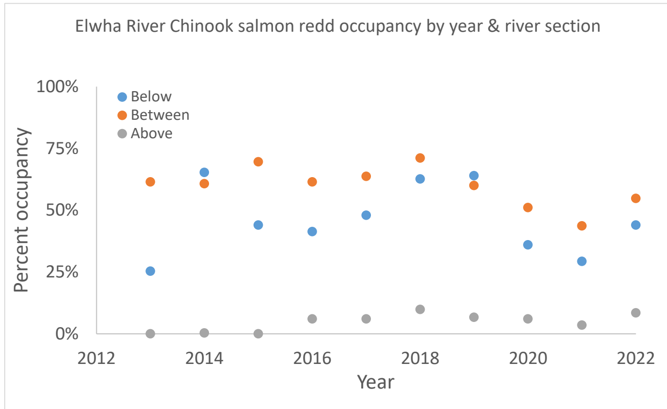
Figure 15. Chinook salmon redd occupancy by year. Chinook salmon redd location was identified to the nearest tenth of a Rkm surveyed from 2012 to 2022 to estimate the total percent linear occupancy for the lower, middle and upper Elwha River.
